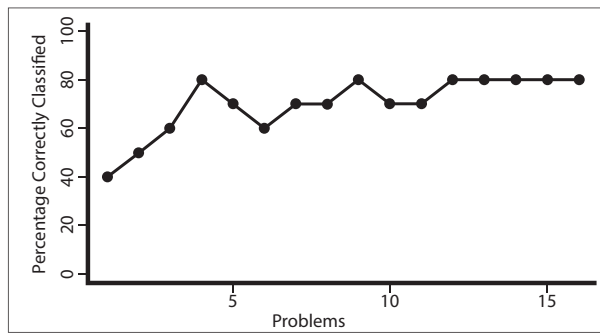
(a) Evolution of Expert Classification
